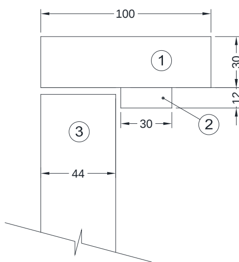
TYPICAL SECTION THROUGH HEAD OF DOOR
