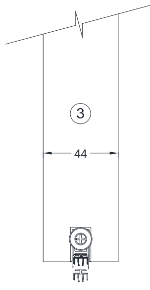
TYPICAL SECTION THROUGH DOOR BASE
