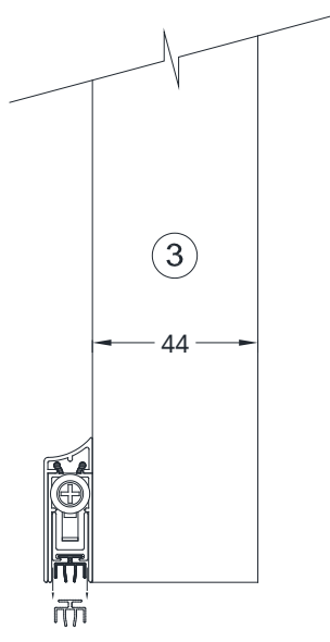
TYPICAL SECTION THROUGH DOOR BASE
