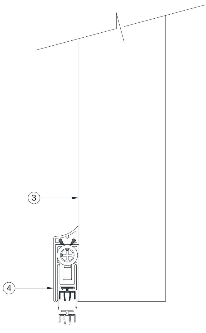
TYPICAL SECTION B - B THROUGH BOTTOM EDGE OF DOOR LEAF
