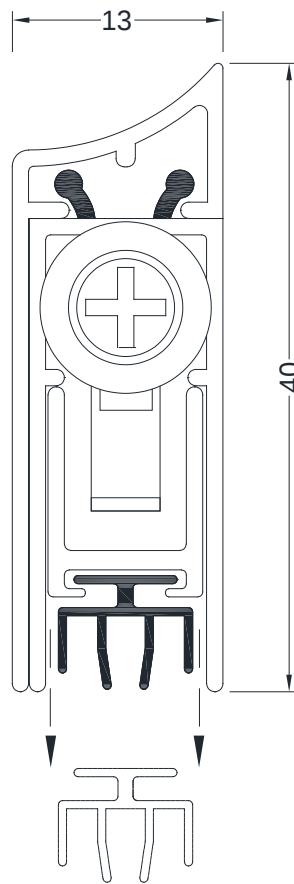
CONCEALEX FACEFIX APPLIQUE
