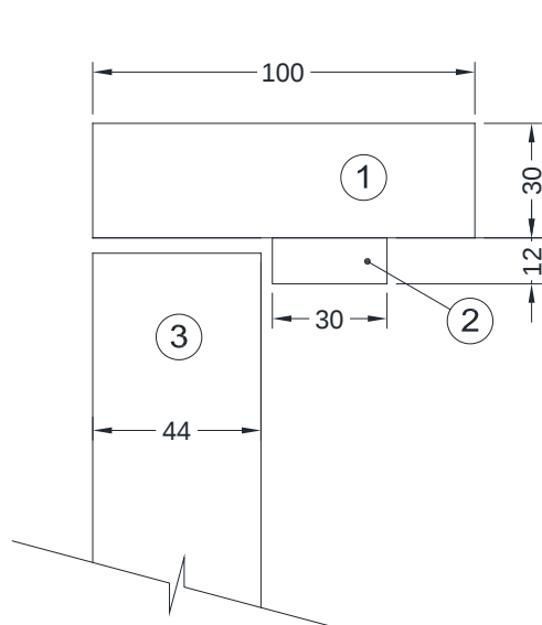
TYPICAL SECTION THROUGH HEAD OF DOOR
